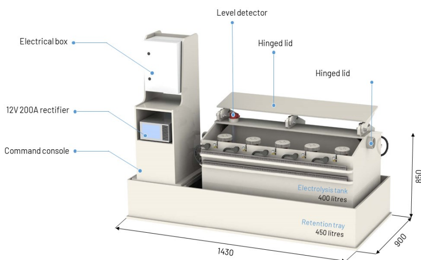
Fig.2 Electrolysis system
